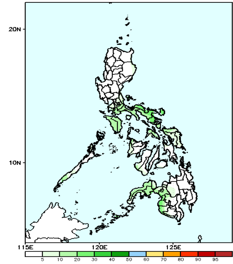
GEFS Week-1 Exceedance Prob. > 150mm Valid: 20241018 - 20241024
