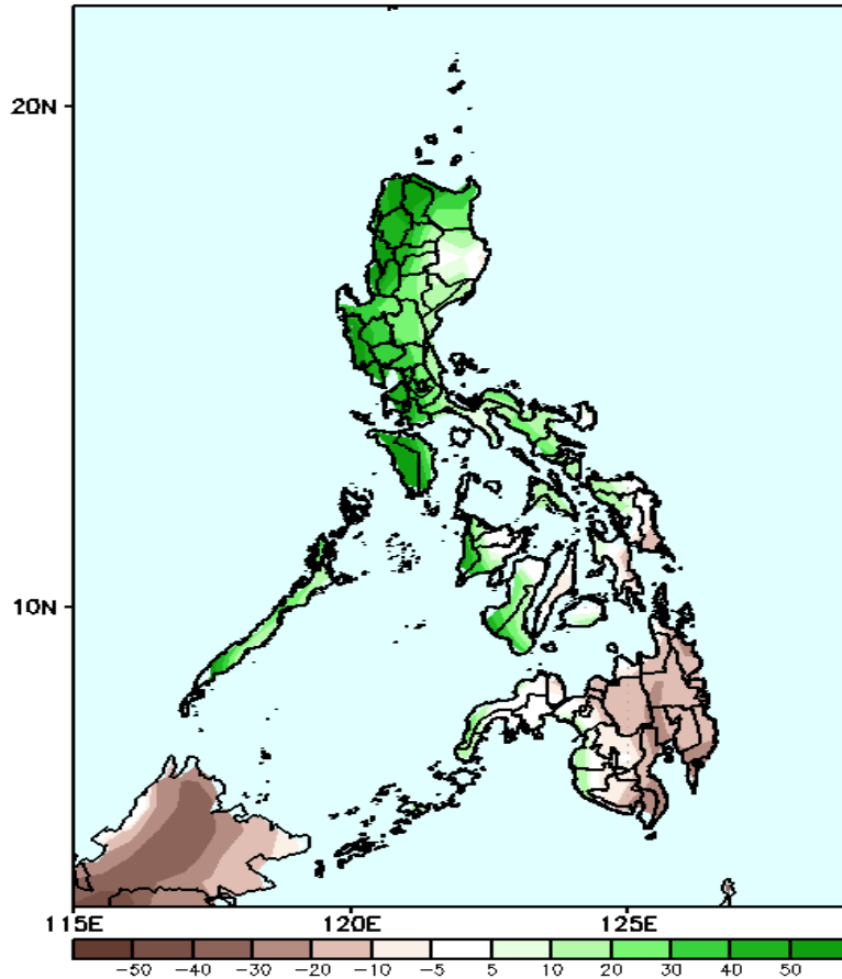
GEFS Week-2 Precip Anomaly Valid: 20241025 - 20241031
