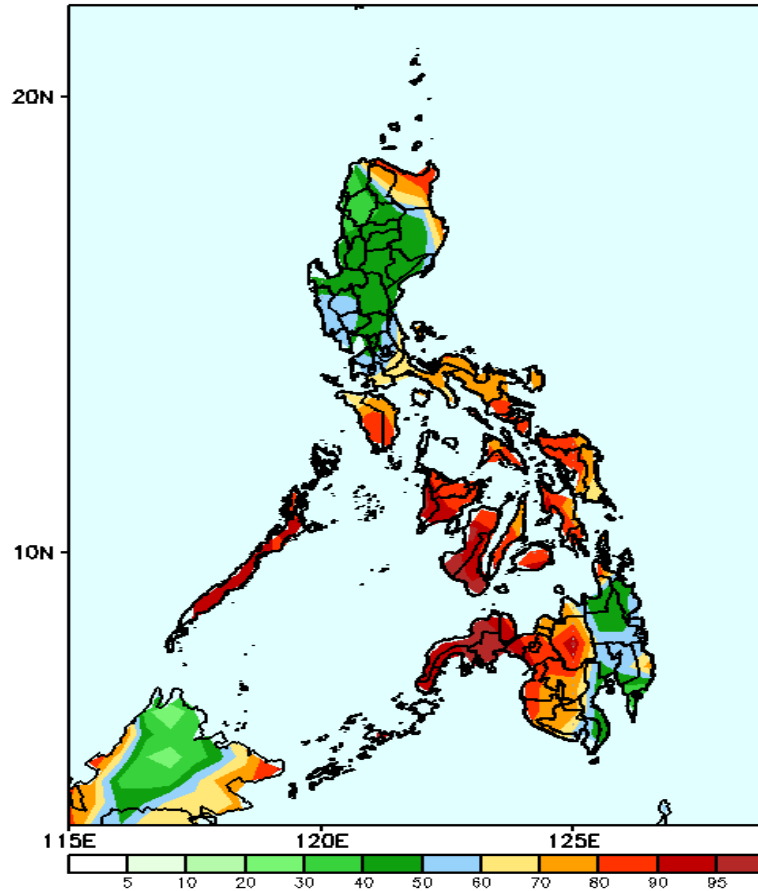
GEFS Week-2 Exceedance Prob. > 25mm Valid: 20241025 - 20241031
