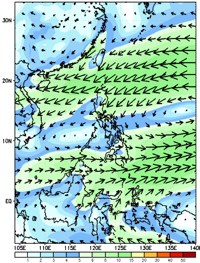
GEFS Week-1 850-hPa Wind Total Valid: 20241018 - 20241024
