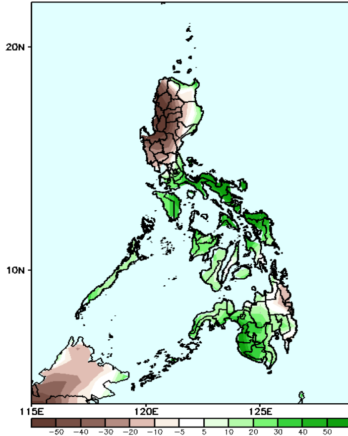
GEFS Week-1 Precip Anomaly Valid: 20241018 - 20241024
