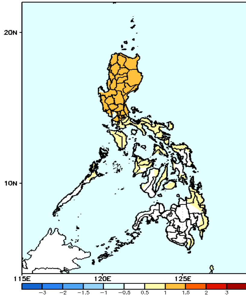
GEFS Week-1 T2m Anomaly Valid: 20241018 - 20241024
