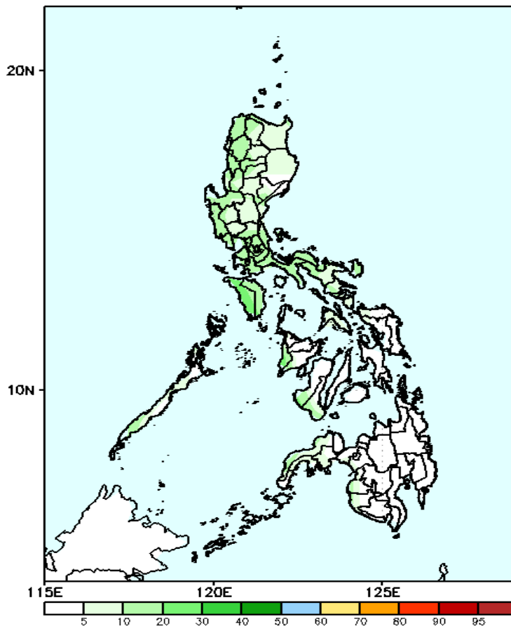
GEFS Week-2 Exceedance Prob. > 150mm Valid: 20241025 - 20241031
