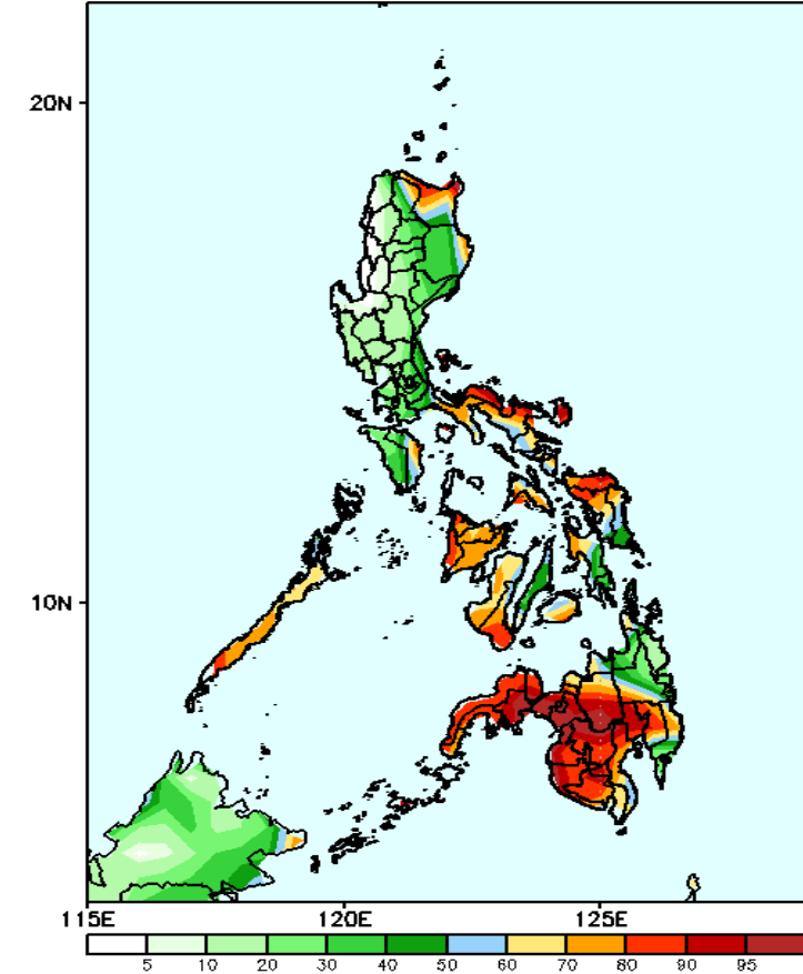
GEFS Week-1 Exceedance Prob. > 50mm Valid: 20241018 - 20241024
