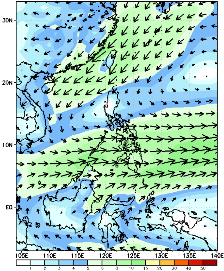
GEFS Week-2 850-hPa Wind Total Valid: 20241025 - 20241031
