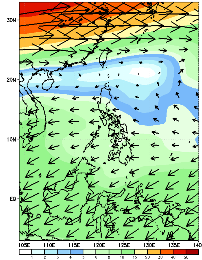
GEFS Week-1 200-hPa Wind Total Valid: 20241018 - 20241024
