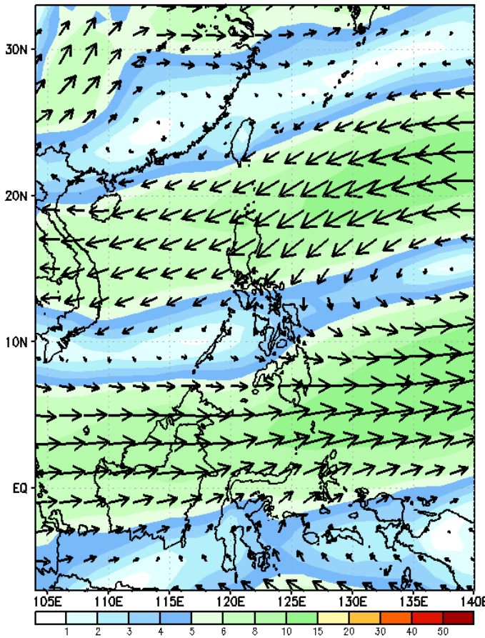
GEFS Week-1 700-hPa Wind Total Valid: 20241018 - 20241024
