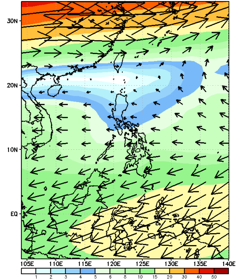
GEFS Week-2 200-hPa Wind Total Valid: 20241025 - 20241031
