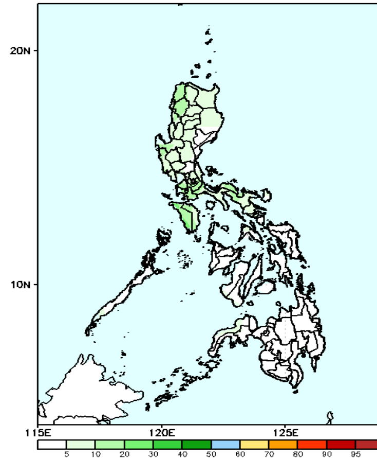
GEFS Week-2 Exceedance Prob. > 200mm Valid: 20241025 - 20241031
