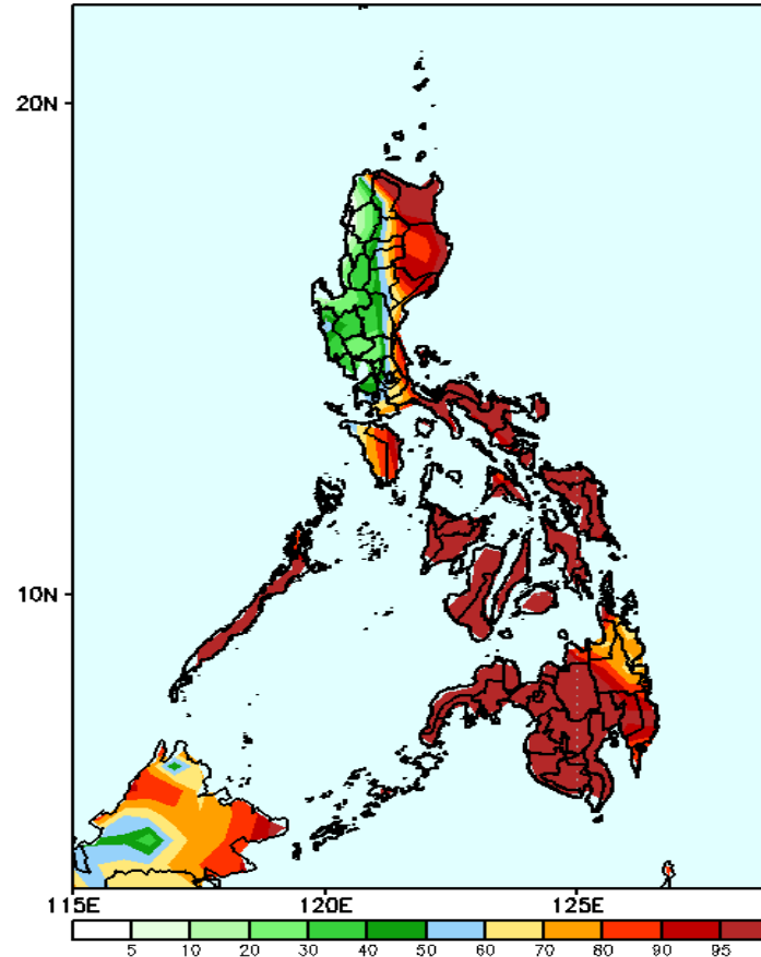
GEFS Week-1 Exceedance Prob. > 25mm Valid: 20241018 - 20241024
