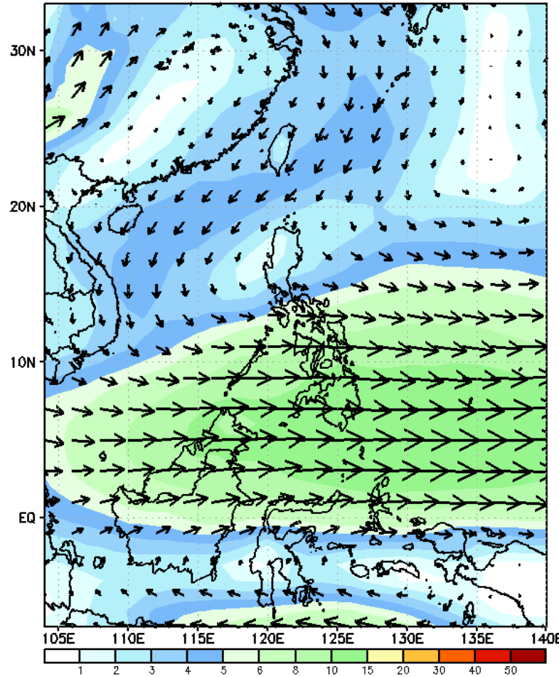
GEFS Week-2 700-hPa Wind Total Valid: 20241025 - 20241031
