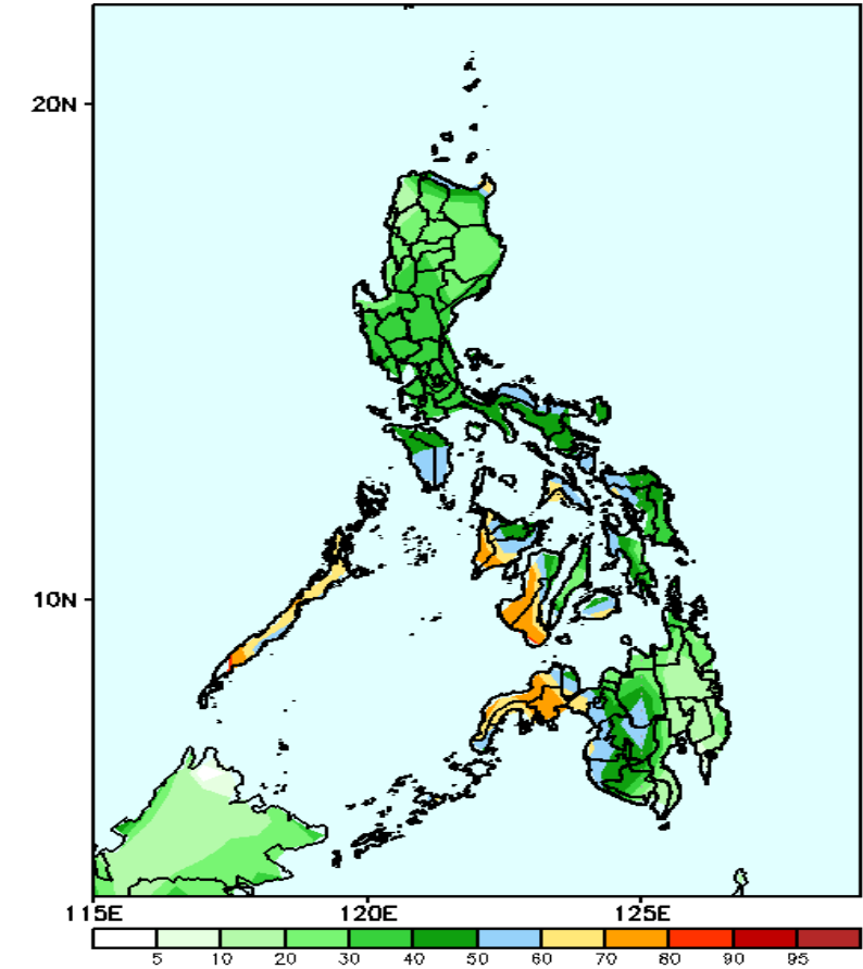
GEFS Week-2 Exceedance Prob. > 50mm Valid: 20241025 - 20241031
