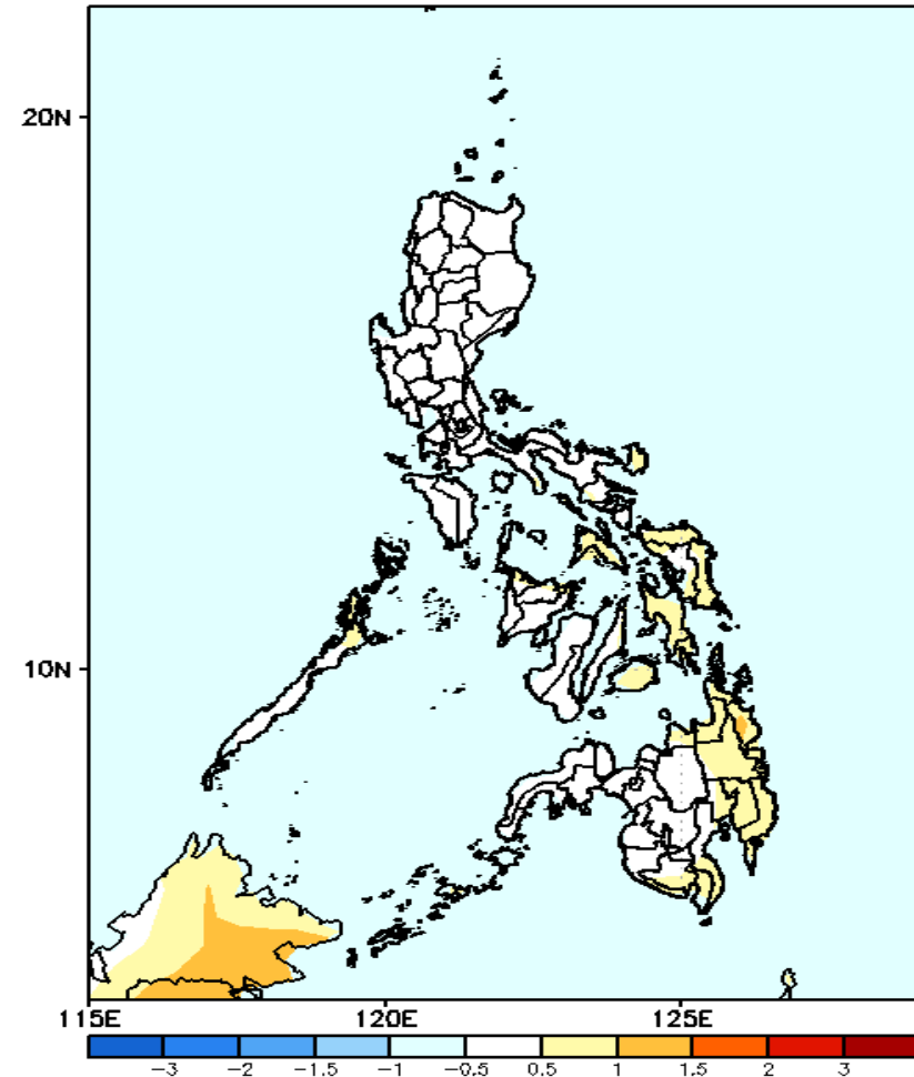
GEFS Week-2 T2m Anomaly Valid: 20241025 - 20241031
