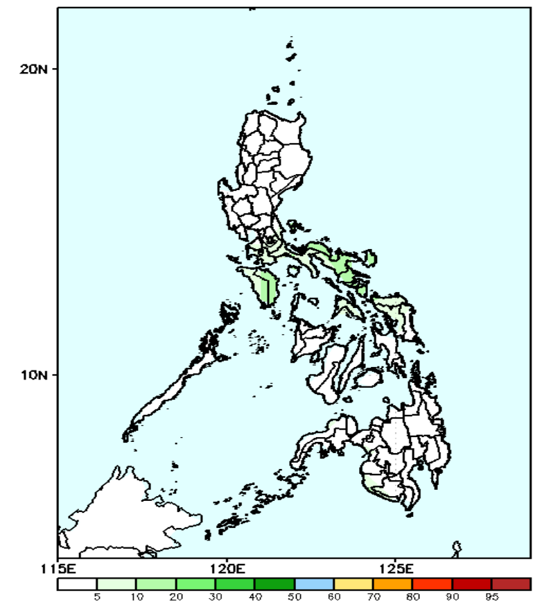
GEFS Week-1 Exceedance Prob. > 200mm Valid: 20241018 - 20241024
