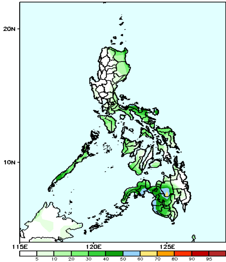
GEFS Week-1 Exceedance Prob. > 100mm Valid: 20241018 - 20241024
