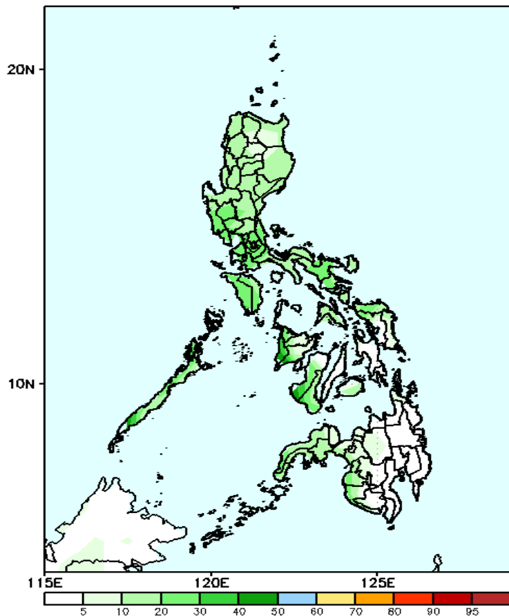
GEFS Week-2 Exceedance Prob. > 100mm Valid: 20241025 - 20241031
